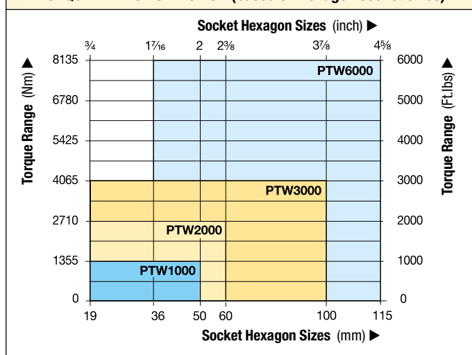
TORQUE WRENCH SELECTION (based on hexagon socket sizes)
