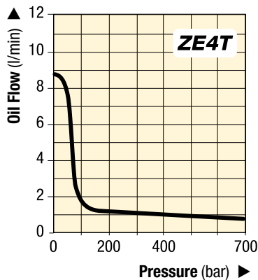
ZE4T AND ZE5T-SERIES OIL FLOW VERSUS PRESSURE
